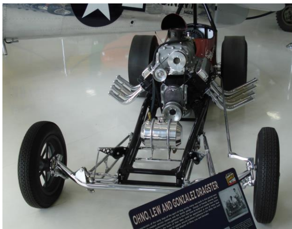
Ohno, Lew & Gonzalez dragster next to a North American Aviation AT-6F/SNJ-6 "Texan" Trainer
