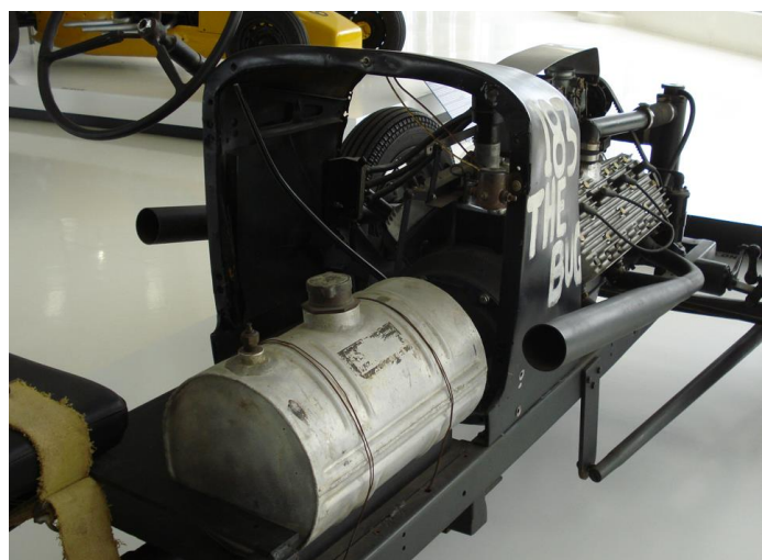
Fuel tank next to driver, no firewall
